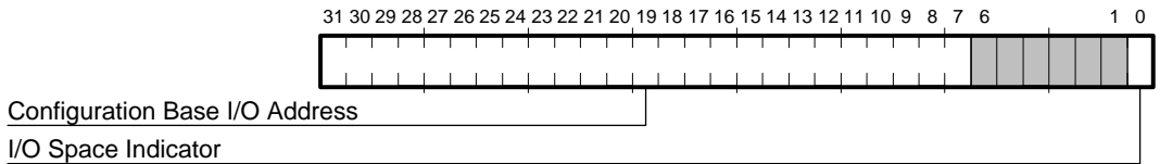
Figure 3–7 CBIO Register Bit Fields
