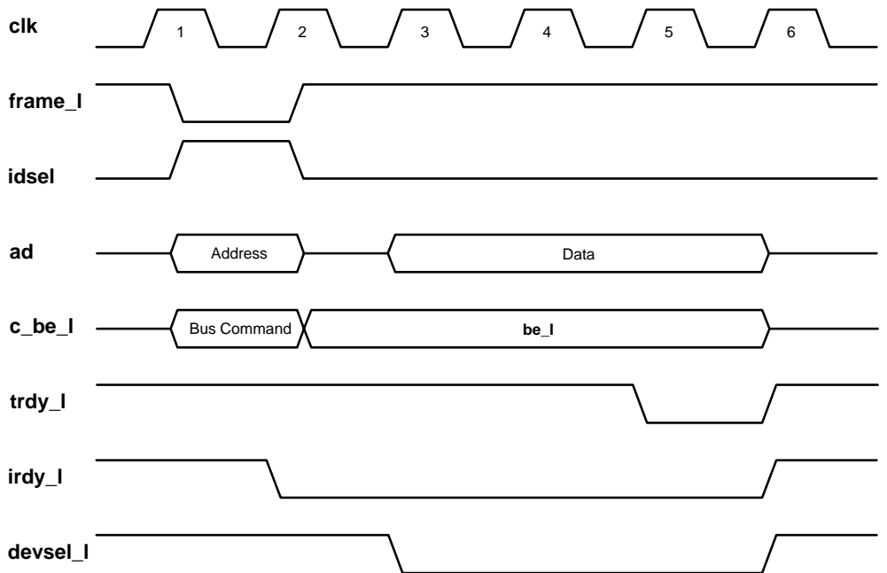
Figure 5–3 Configuration Read Cycle
