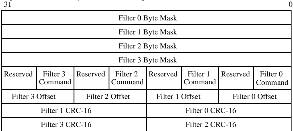
Figure 3–25 Wake-Up Frame Filter Register Structure
