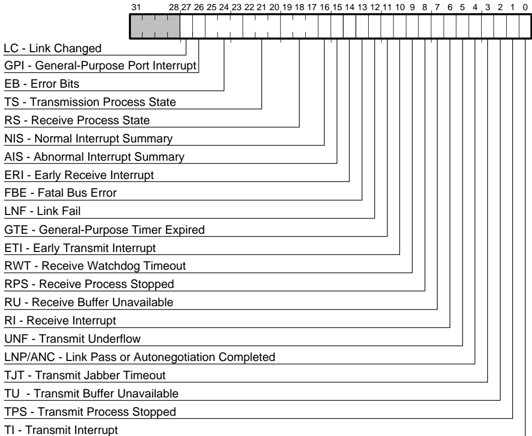
Figure 3–34 CSR5 Register Bit Fields
