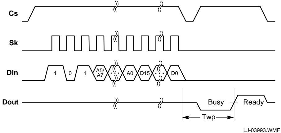
Figure 8–10 Write Operation
