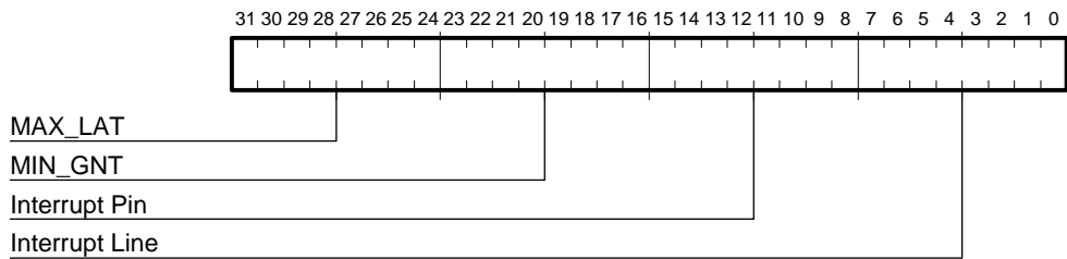
Figure 3–13 CFIT Register Bit Fields
