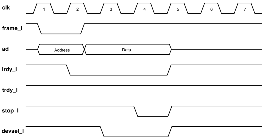
Figure 5–8 21143-Initiated Retry Cycle
