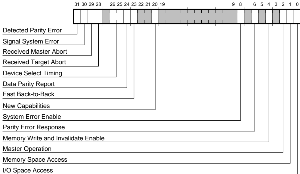
Figure 3–4 CFCS Register Bit Fields
