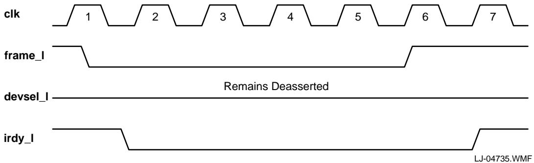
Figure 5–10 Master Abort
