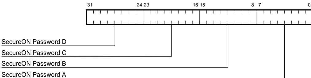
Figure 3–19 SOP0 Register Bit Fields
