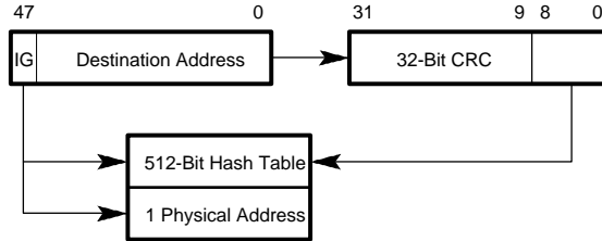
Figure 4–13 Imperfect Filtering
