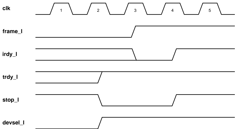
Figure 5–11 Target Abort
