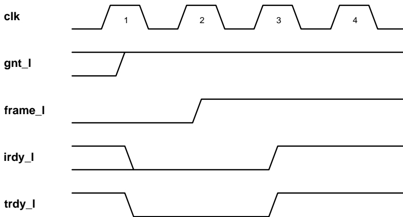
Figure 5–9 Normal Completion
