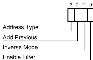
Figure 3–27 Filter i Command Bit Fields
