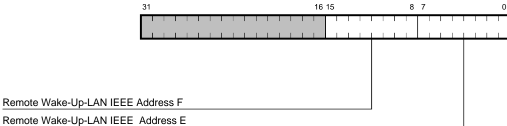
Figure 3–18 CWUA1 Register Bit Fields
