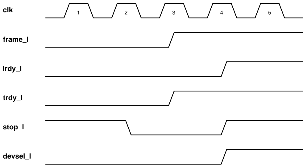
Figure 5–12 Target Disconnect
