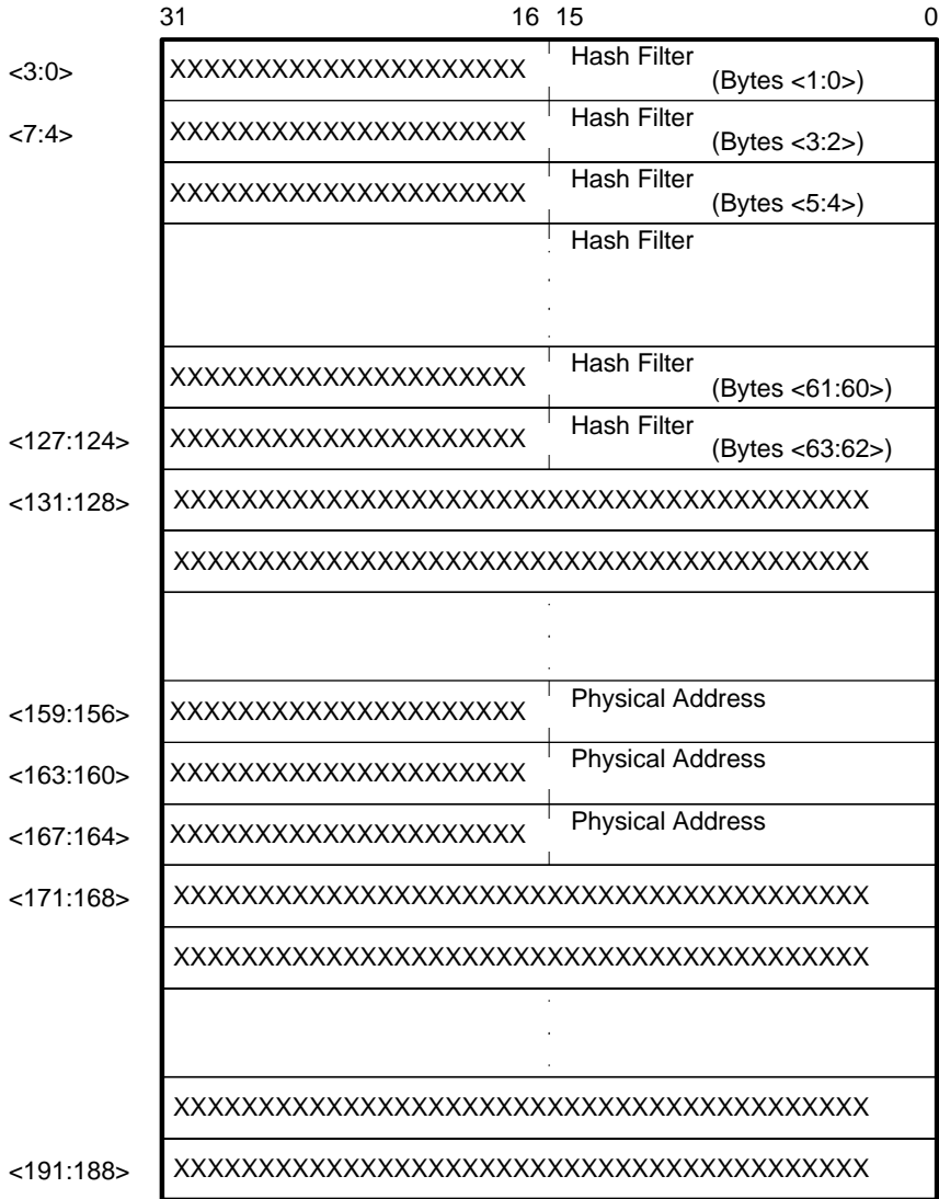
Figure 4–14 Imperfect Filtering Setup Frame Buffer Format
