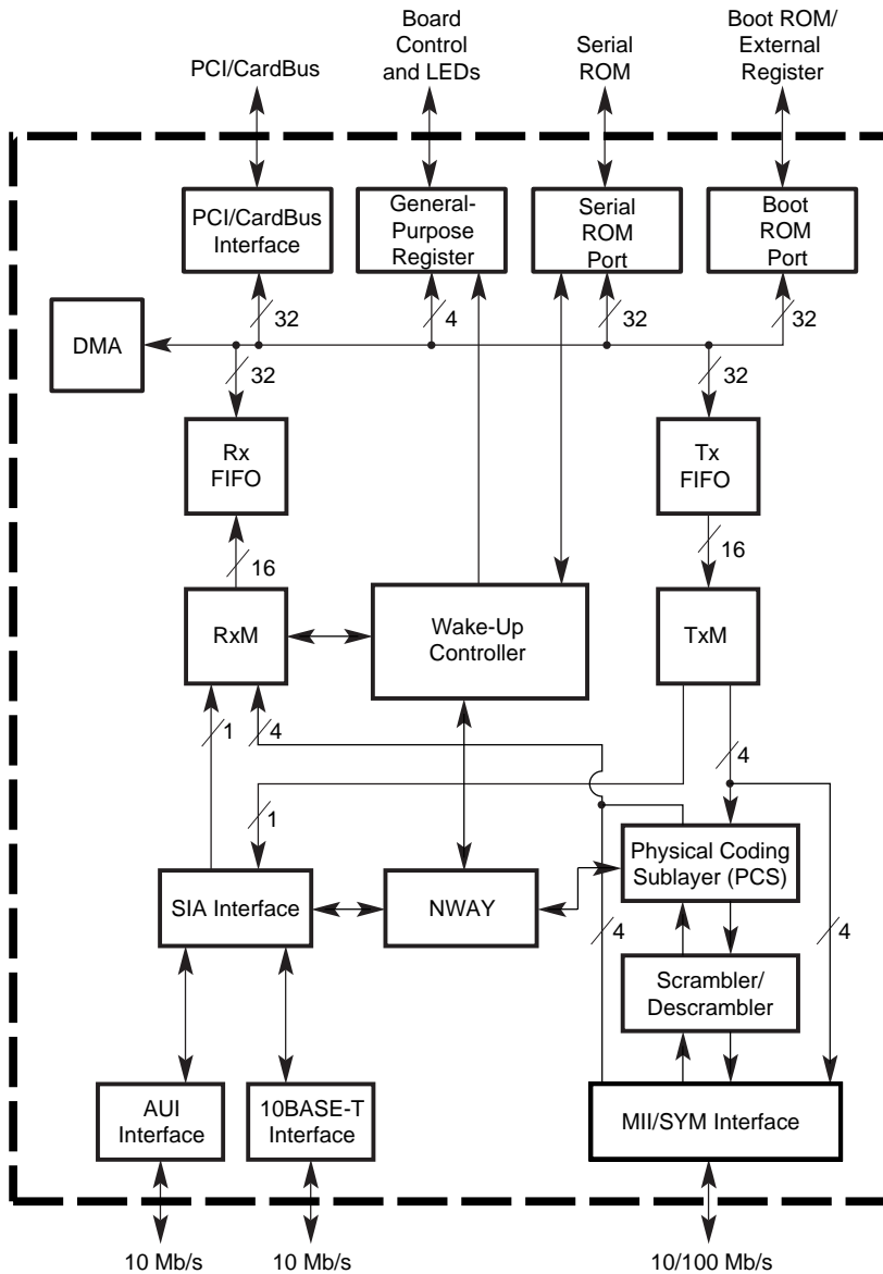
Figure 1-1 21143 Block Diagram
