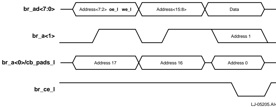
Figure 8–3 Boot ROM Byte Write Cycle
