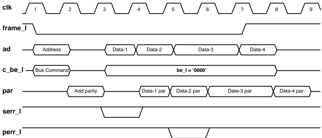
Figure 5–14 Parity Operation
