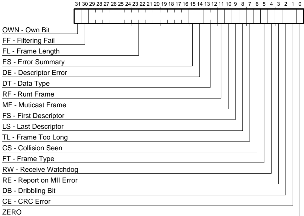
Figure 4–3 RDES0 Bit Fields
