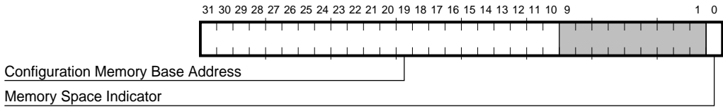
Figure 3–8 CBMA Register Bit Fields
