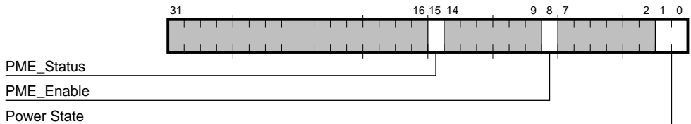
Figure 3–15 CPMC Register Bit Fields
