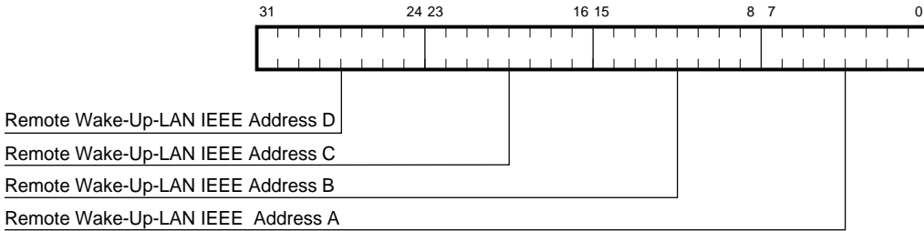
Figure 3–17 CWUA0 Register Bit Fields
