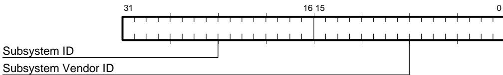
Figure 3–10 CSID Register Bit Fields
