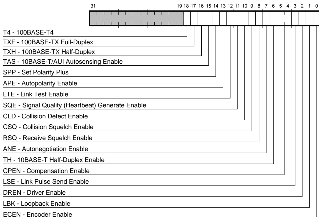
Figure 3–43 CSR14 Register Bit Fields
