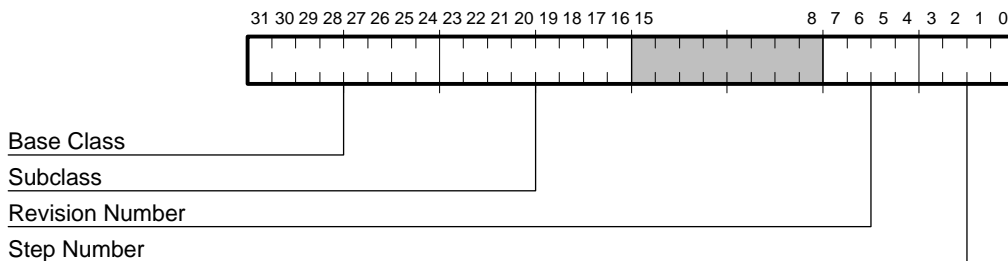
Figure 3–5 21143 CFRV Register Bit Fields
