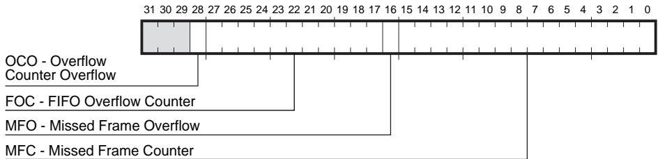
Figure 3–37 CSR8 Missed Frames and Overflow Counter
