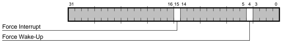
Figure 3–48 FFER Register Bit Fields
