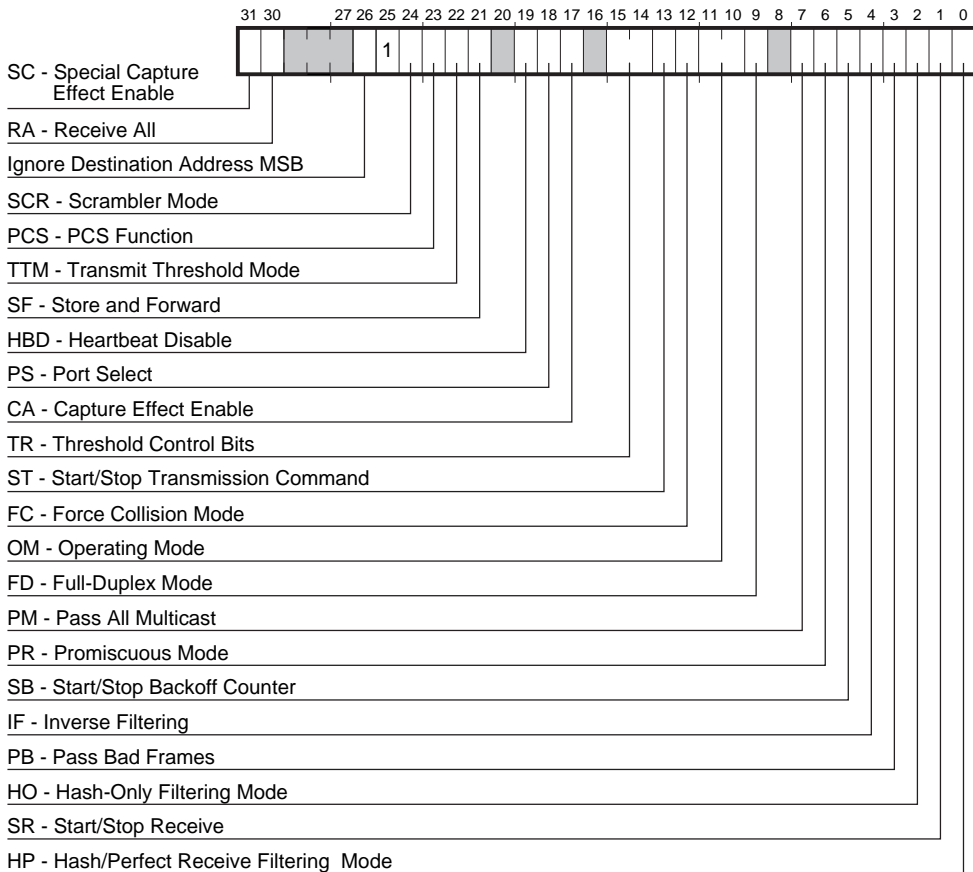
Figure 3–35 CSR6 Register Bit Fields
