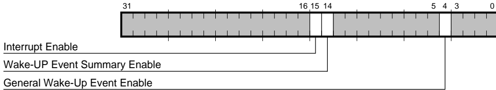
Figure 3–46 FEMR Register Bit Fields
