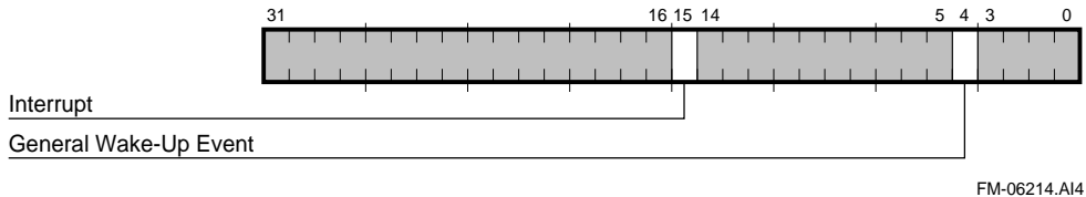
Figure 3–45 FER Register Bit Fields
