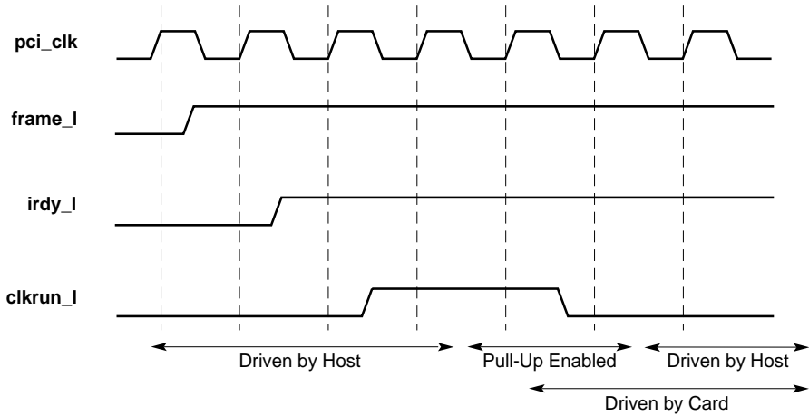
Figure 5–16 PCI/CardBus Clock—Maintaining Speed
