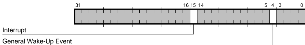
Figure 3–47 FPSR Register Bit Fields
