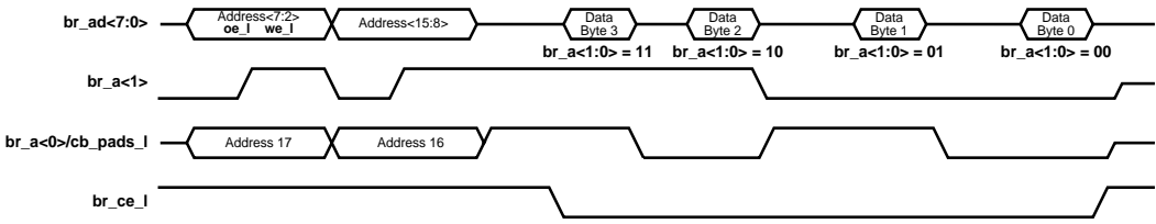
Figure 8–4 Boot ROM Dword Read Cycle
