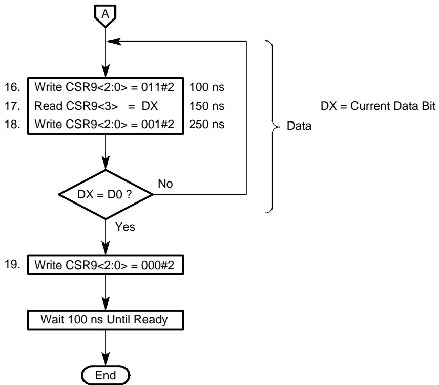
Figure 8–6 Read Cycle (Page 2 of 2)
