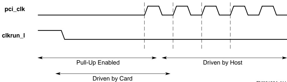
Figure 5–15 PCI/CardBus Clock—Restart or Speed-Up
