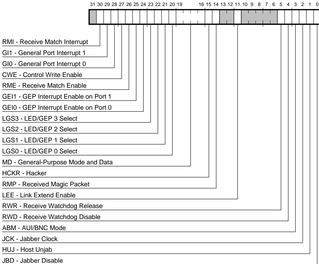
Figure 3–44 CSR15 Register Bit Fields
