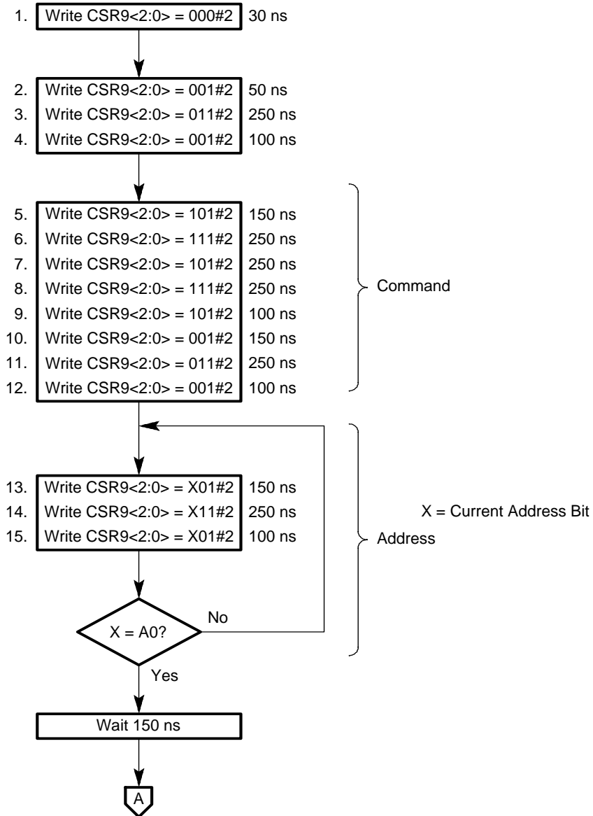
Figure 8–5 Read Cycle (Page 1 of 2)
