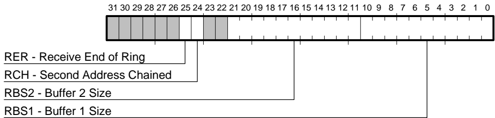
Figure 4–4 RDES1 Bit Fields
