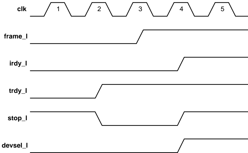
Figure 5–13 Target Retry
