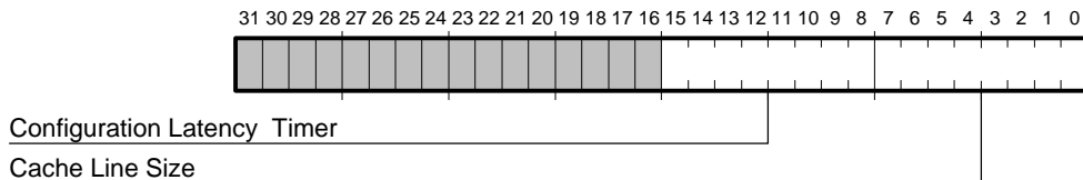
Figure 3–6 CFLT Configuration Latency Timer Register
