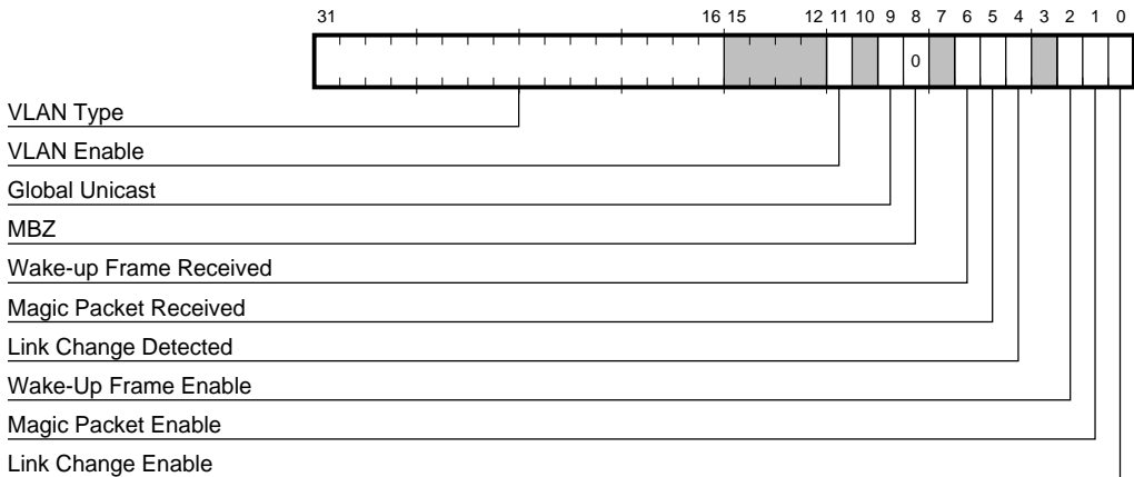
Figure 3–31 CSR2-PM Register Bit Field
