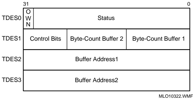
Figure 4-7 Transmit Descriptor Format
