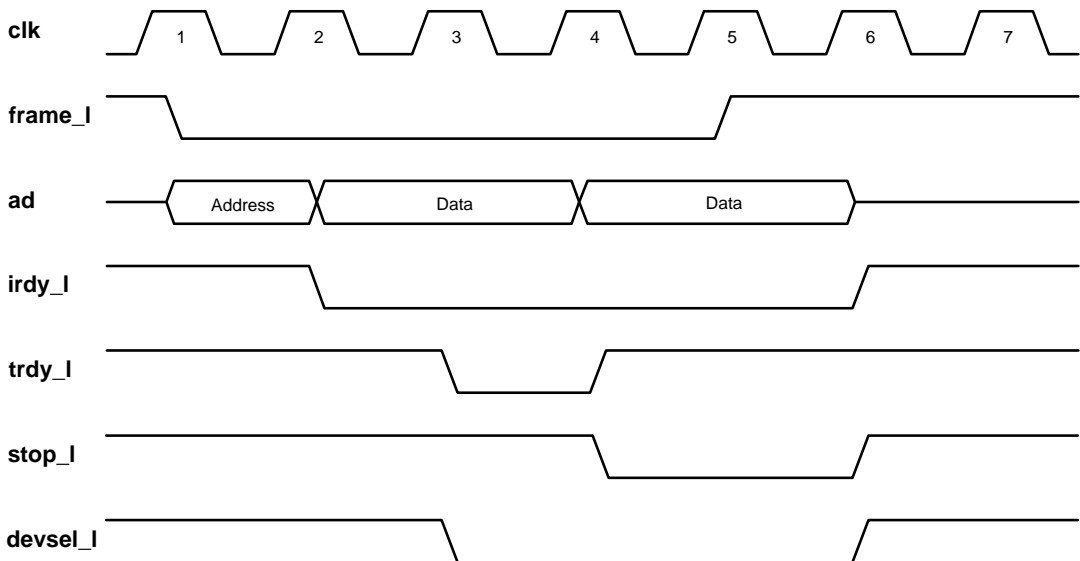
Figure 5–7 21143-Initiated Disconnect Cycle
