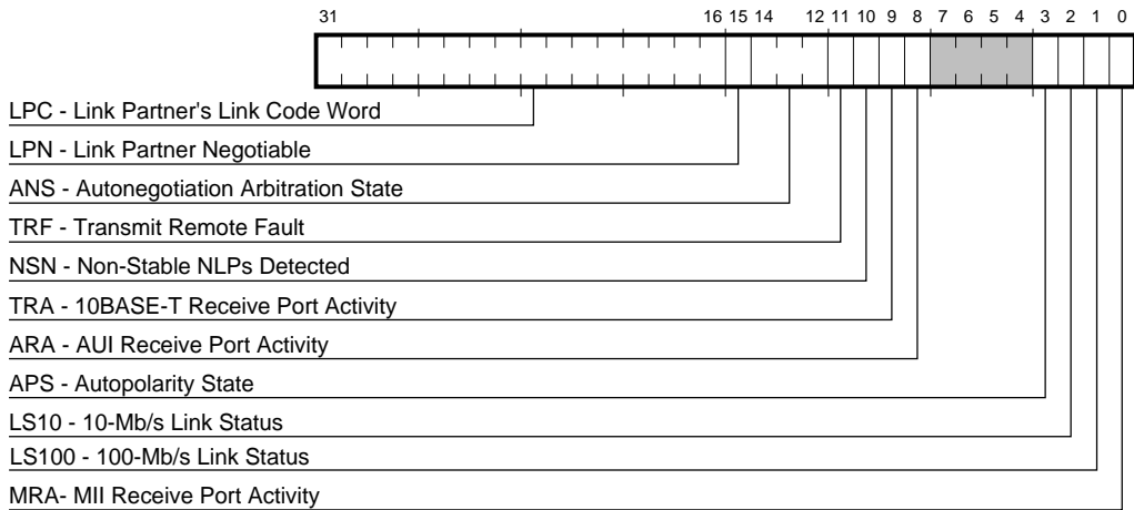
Figure 3–41 CSR12 Register Bit Fields
