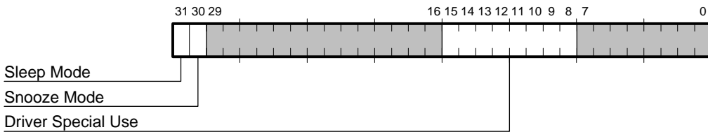
Figure 3–16 CFDD Register Bit Fields
