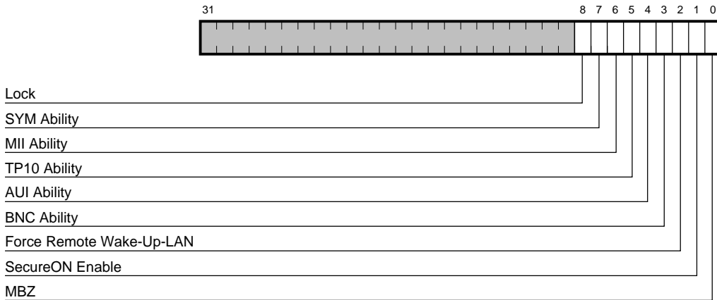
Figure 3–21 CWUC Register Bit Fields
