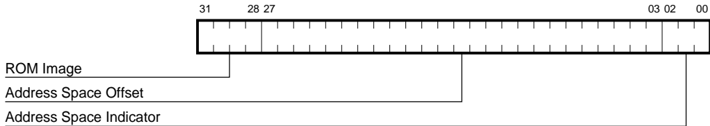
Figure 3–9 CCIS Register Bit Fields
