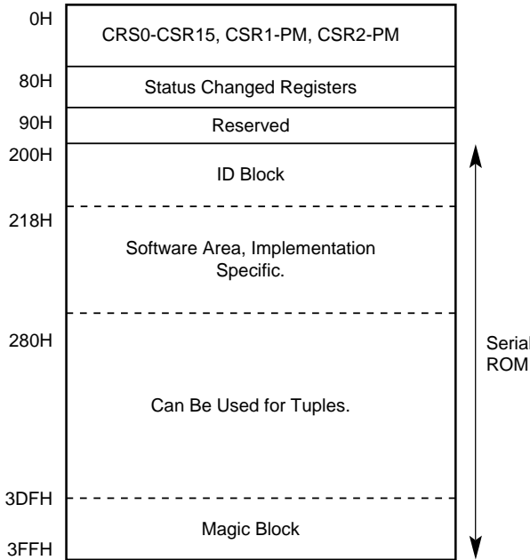
Figure 3–1 21143 Memory Map
